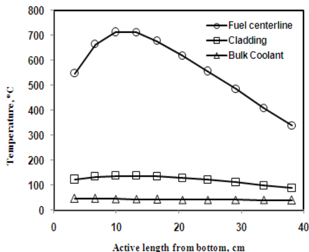
Fig. 7. Axial temperature distribution in the hottest channel of C10 at 700 MWD burnt condition.
