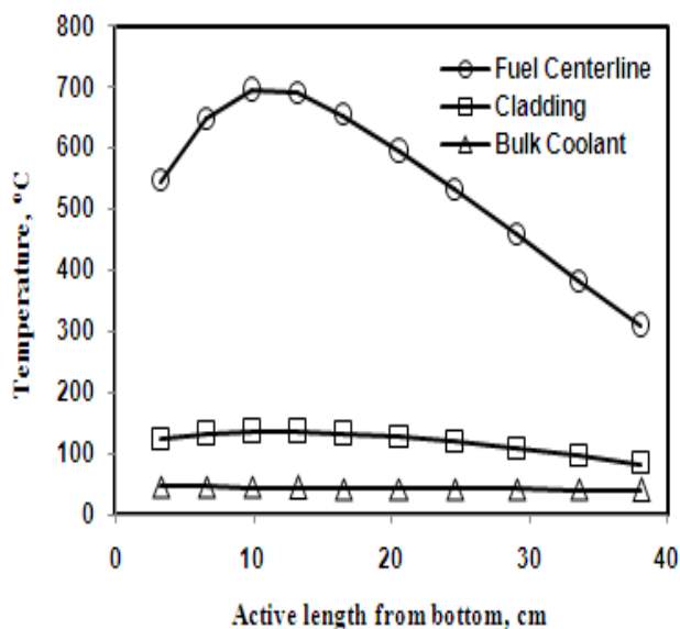
Fig. 6. Axial temperature distribution in the hottest channel of C4 at 150 MWD burnt condition.
