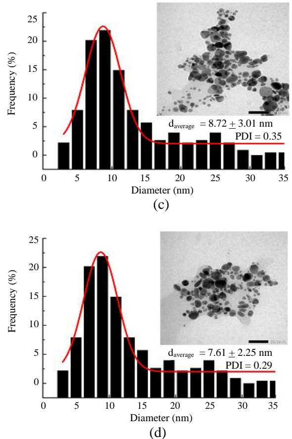
Fig. 5. TEM micrograph and particle size distribution of AgNPS stabilized in (a) 0.05, (b) 0.1, (c) 0.5, and (d) 1.0 % (w/v) i-carrageenan
