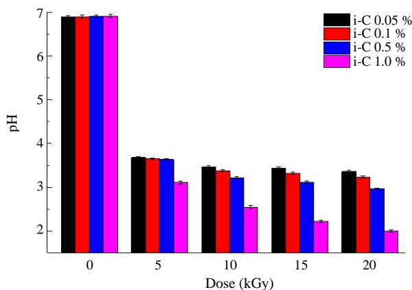
Fig. 6. pH of ι-carrageenan irradiated at various doses.
