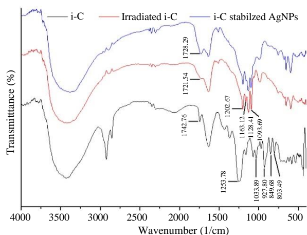
Fig. 3. FTIR spectra of raw \iota -carrageenan, irradiated \iota -carrageenan, and \iota -carrageenan supported AgNPs.
