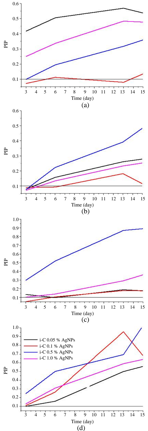
Fig. 7. Particle instability parameter of ι-carrageenan supported AgNPs synthesized at \gamma -ray dose of (a) 5, (b) 10, (c) 15 and (d) 20 kGy at function of time.
